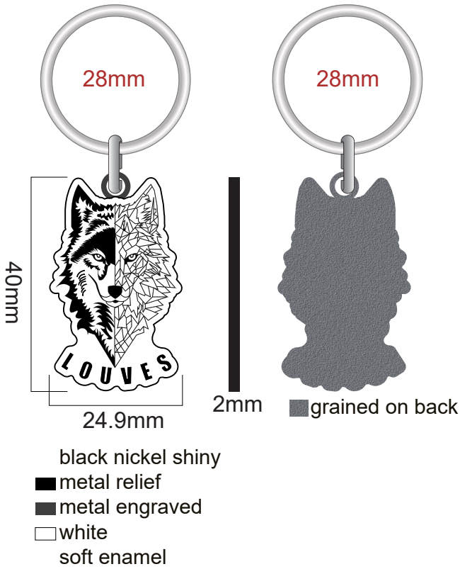
ZINCALLOY KEYCHAIN
