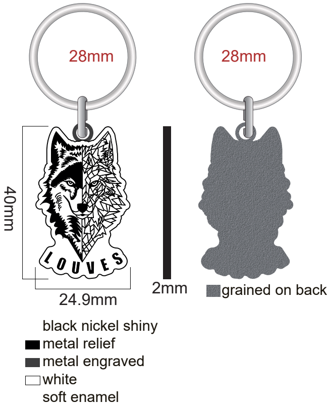
ZINCALLOY KEYCHAIN
